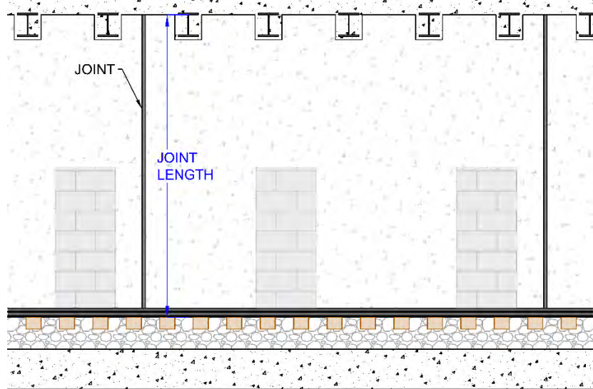
TUNNEL LONGITUDINAL SECTION
