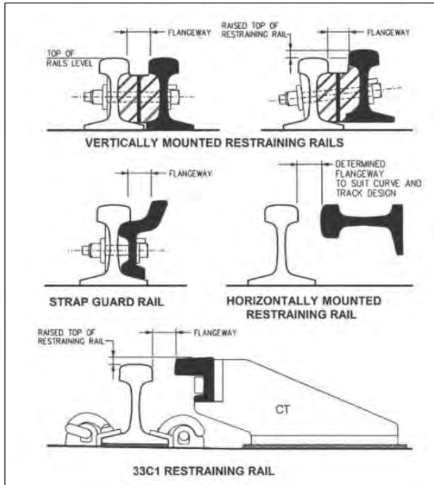
Figure 6.6.3-4 Types of Restraining Rails
