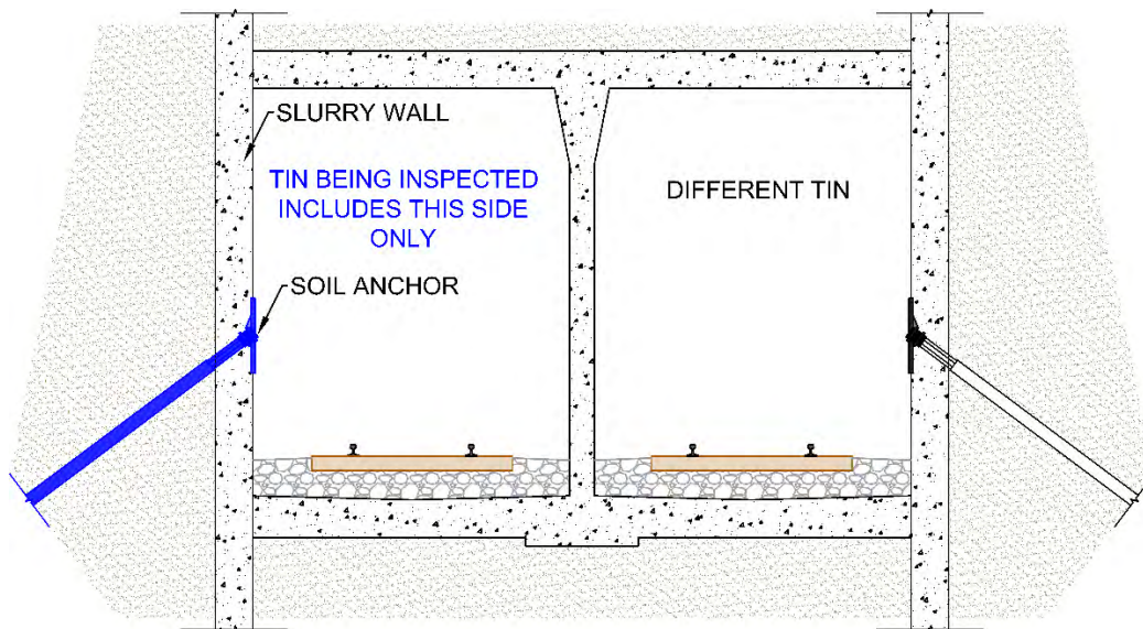
Figure 7.3.4-12 Element Qty Boundary: Soil Anchor (EA)
