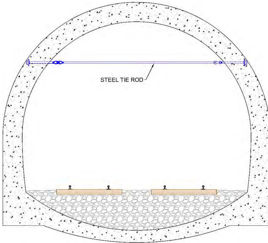
TUNNEL CROSS SECTION
