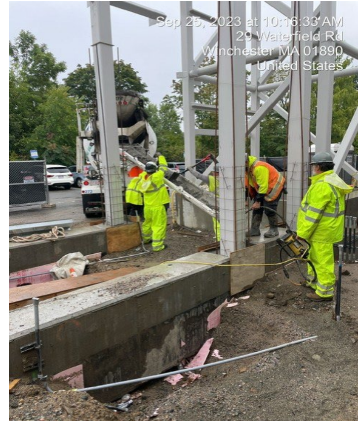
Concrete placement at East Headhouse Columns (September 2023)
