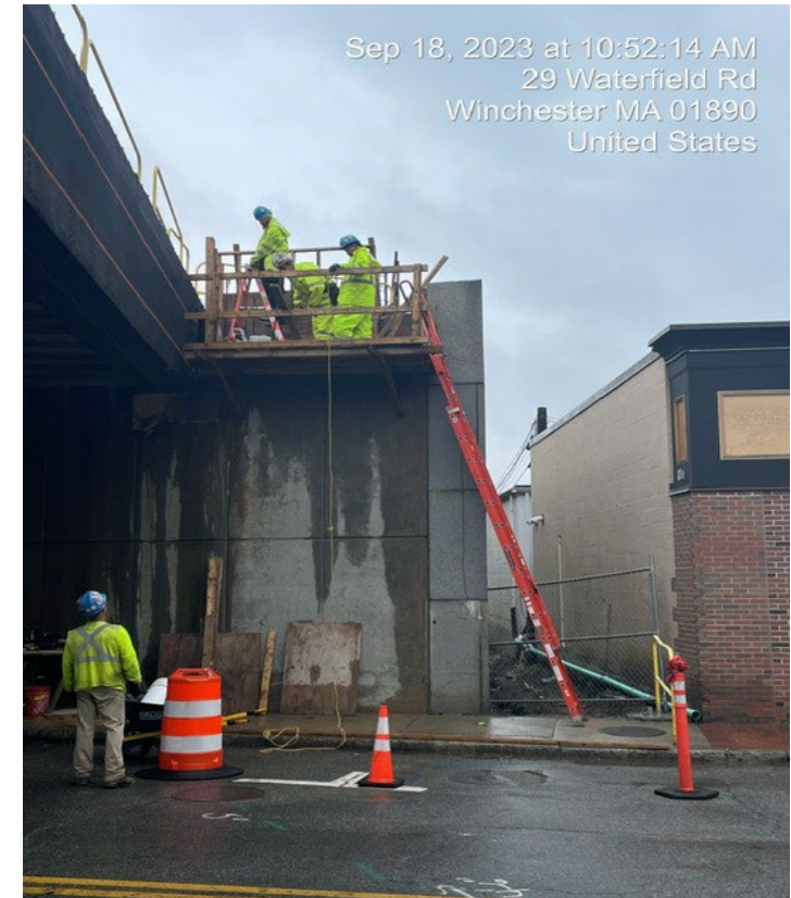
Abutment Cap Construction Outbound Platform – along Waterfield Road (September 2023)
